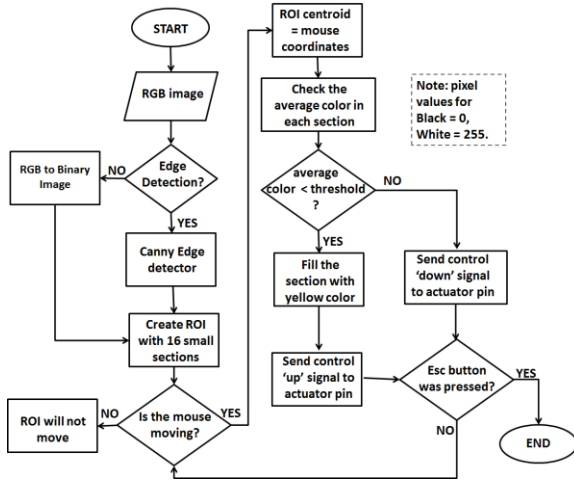
Fig. 5. Tactile display simulator flowchart.
