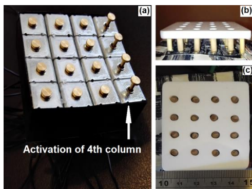
Fig. 3. Prototype 1: 4x4 Tactile Display. (a) 4th column activated, (b) wooden pins are put on top of each plunger to insulate the user from the heat dissipated by the solenoids during prolong usage, and (c) top view.
