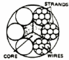
Figure 5A.1-4 Wire Rope Construction
